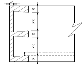
Lapped dovetail
