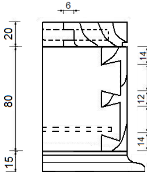
JOINT DETAIL AT BACK
